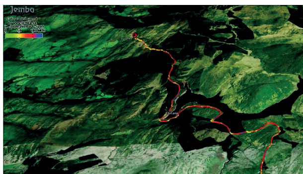
Speed trace before recommendations.
